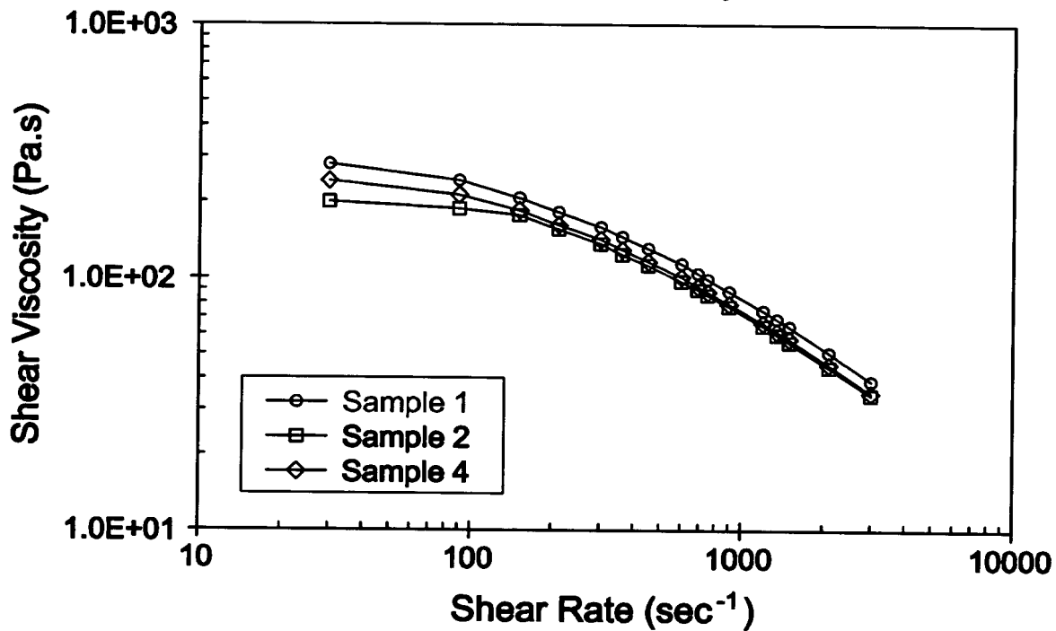
Fig. 11 Shear Viscosity of Plasticized Metallocene Propylene Homopolymers
